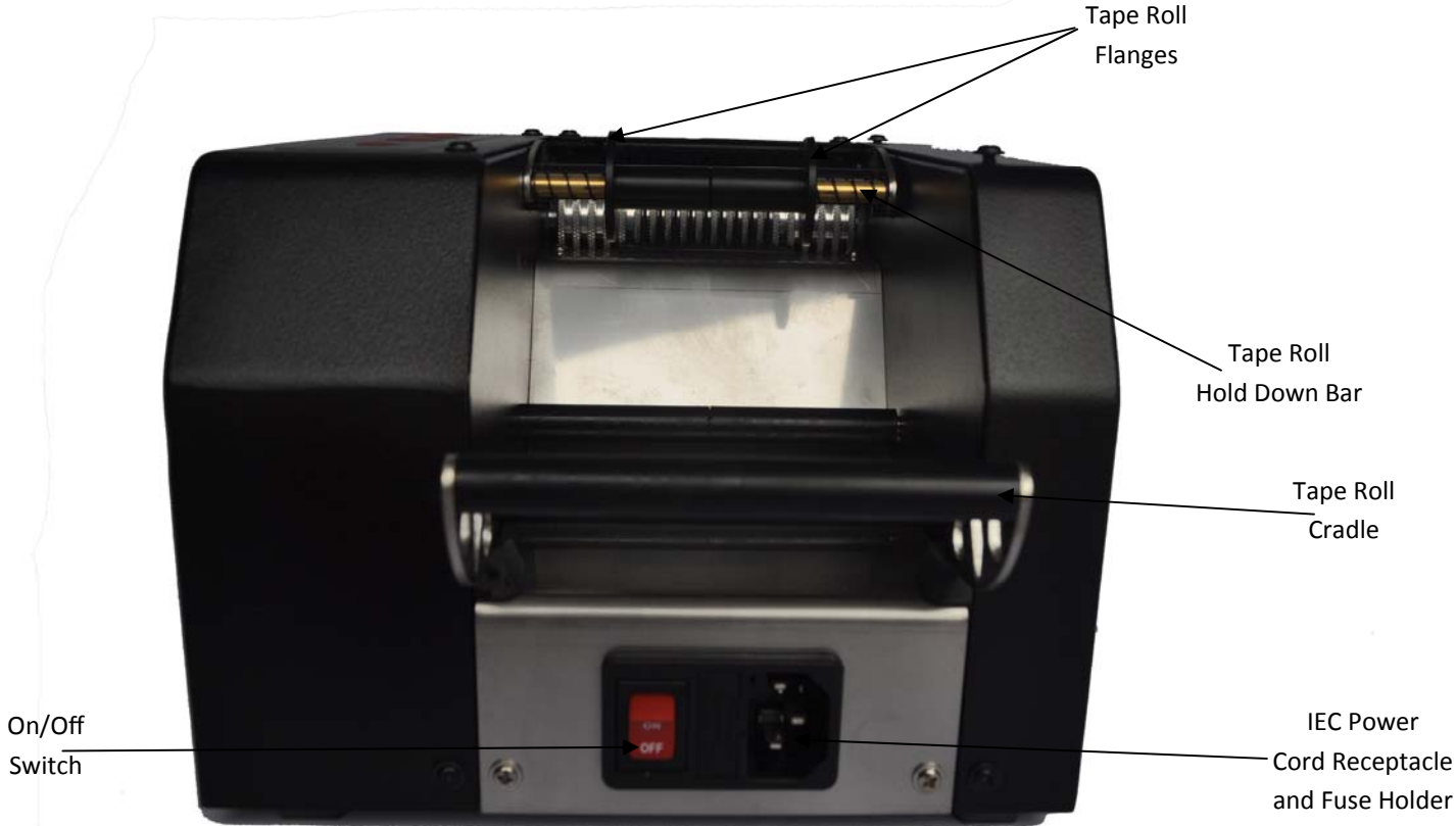
Figure 3 Front View: ↓
